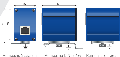
MJ8-POE-C6A
